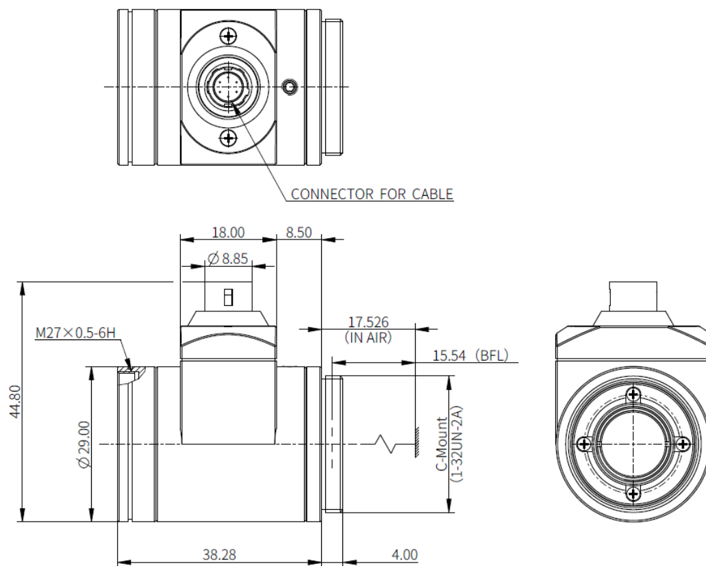
Figure 1: Mechanical drawing of the ELM-35-6.4-11-C
